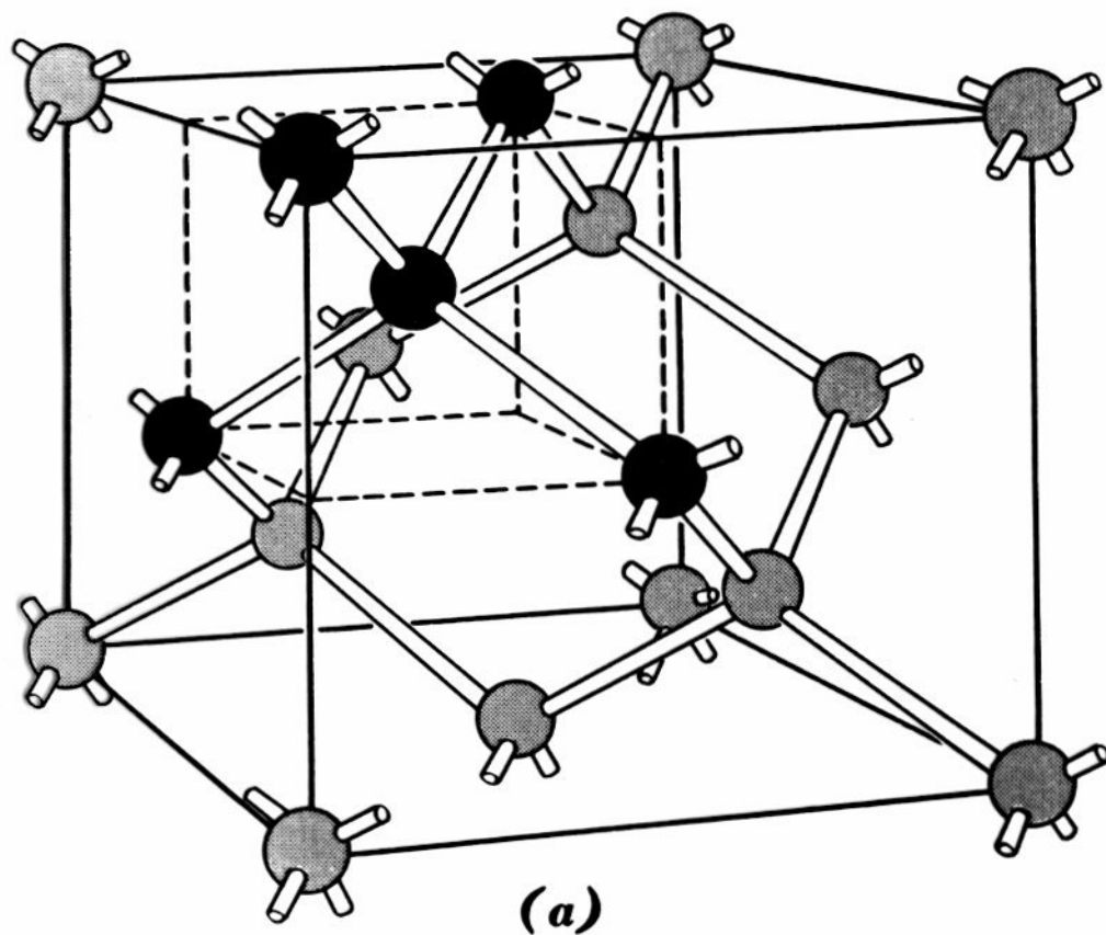
FIGURE 17.4 (a) The tetrahedral structure of diamond. The coordination number is 4. (b) Scale model of diamond crystal.
