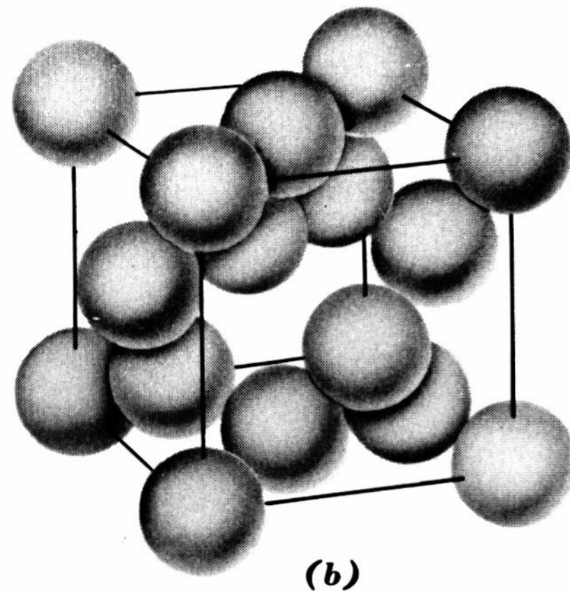
FIGURE 17.4 (a) The tetrahedral structure of diamond. The coordination number is 4. (b) Scale model of diamond crystal.
