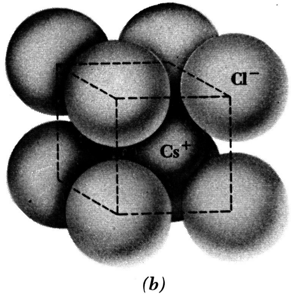
FIGURE 17.3 (a) The body-centered cubic structure of a CsCl crystal. The coordination number is 8. (b) Scale model of CsCl crystal.
