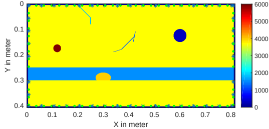
Figure: 2D model with pipe and additional perturbations.
