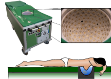
Prototype of a ultrasound device with a full 3D acquisition geometry (Ruiter et al., 2017). (Kühn 2018)
