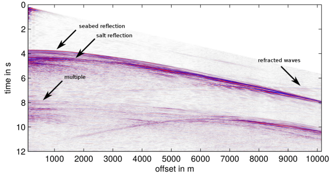
Recorded pressure field at the sea surface
