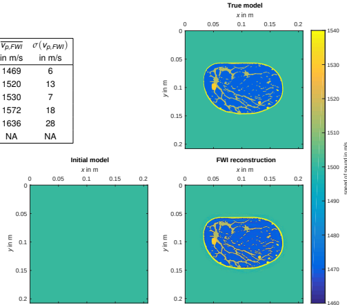
True, initial and inverted speed of sound models (Kühn 2018)
