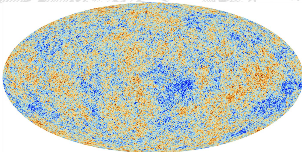
Galactic foregrounds removed
