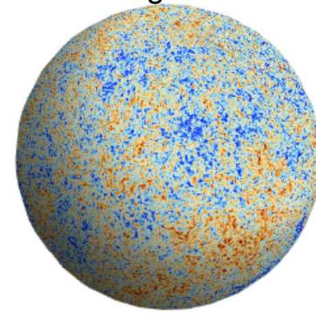
Galactic foregrounds removed
