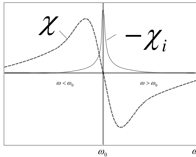
Figure 1. Real and imaginary part of the first order susceptibility.
