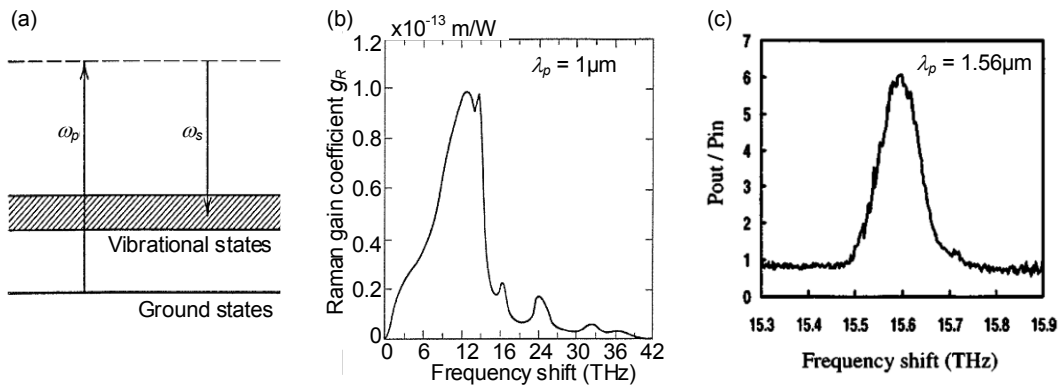
Figure 1: (a) Energy-level representation of SRS. (b) Raman gain spectrum in a fused-silica fiber for a pump wavelength of 1000 nm [1]. (c) Raman gain spectrum in a silicon-on-insulator waveguide for a pump wavelength of 1557.4 nm [2]. Note that on the vertical axis in (b) and (c) two different quantities have been measured and therefore the numbers are not comparable.
